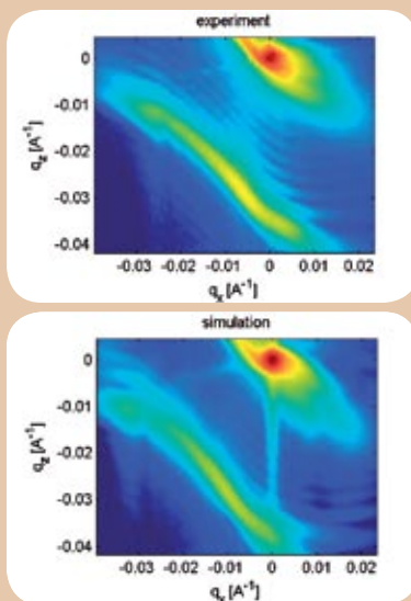
Fig. 6: Measured (top) and simulated (bottom) distribution of diffracted x-ray intensity in reciprocal space, periodic grating of wires lithographically prepared in a thin layer of (Ga,Mn)As.
