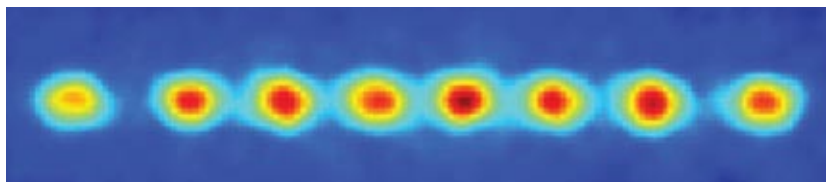
LEVITATED STRING of calcium ions in a vacuum chamber can perform quantum calculations.
